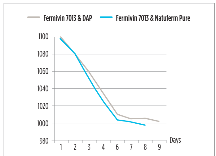
Fermentation kinetics of a Syrah must (in the liquid phase, NTU 328, pH 3.72, Nass 188 mg/l) - Natuferm Pure and DAP added at density - 10 points - DAP at 8 mg/l of YAN vs. Natuferm Pure at 2.5 mg/l of YAN.
